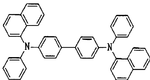
NPB
