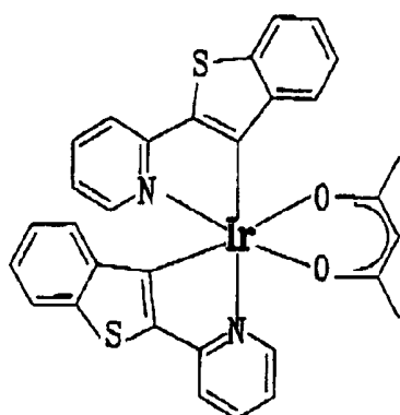
(btp) 2 Ir(acac)
